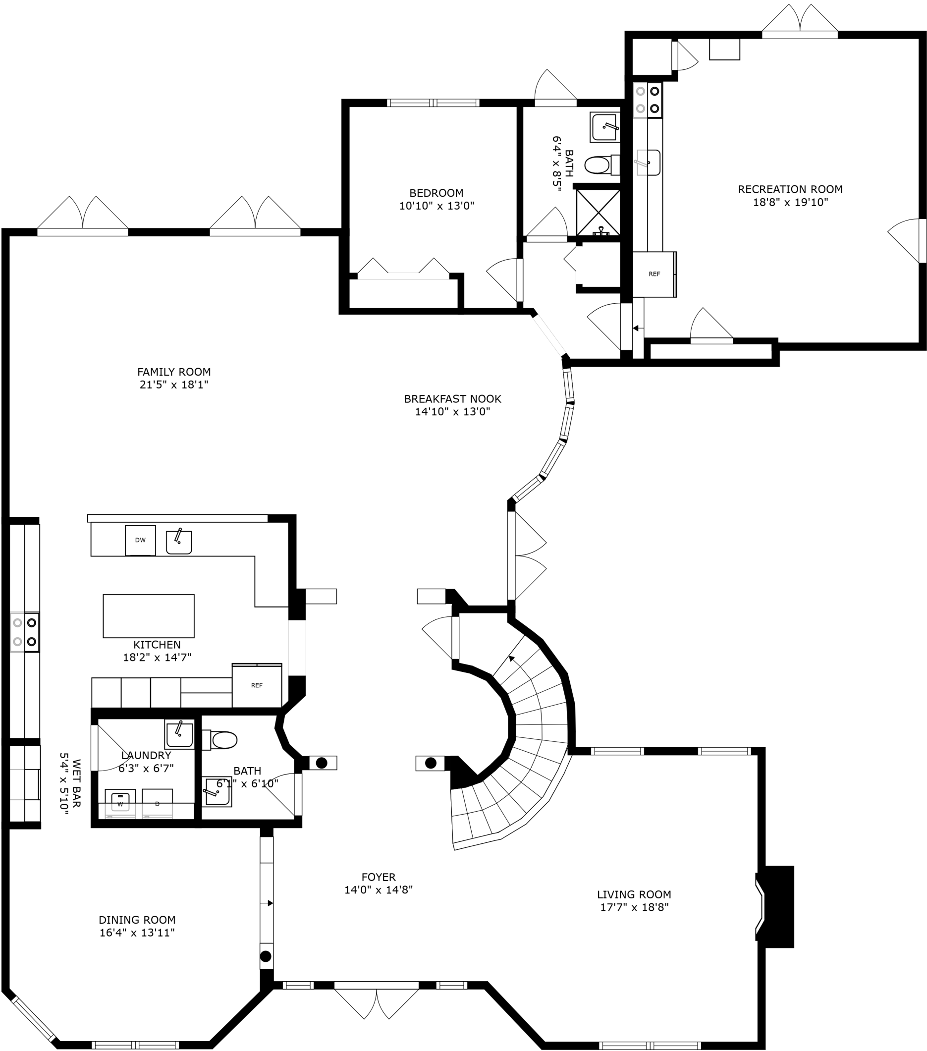
FLOOR 1
