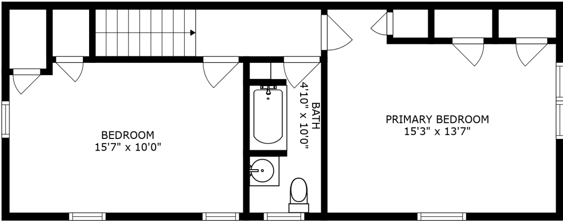
FLOOR 5
