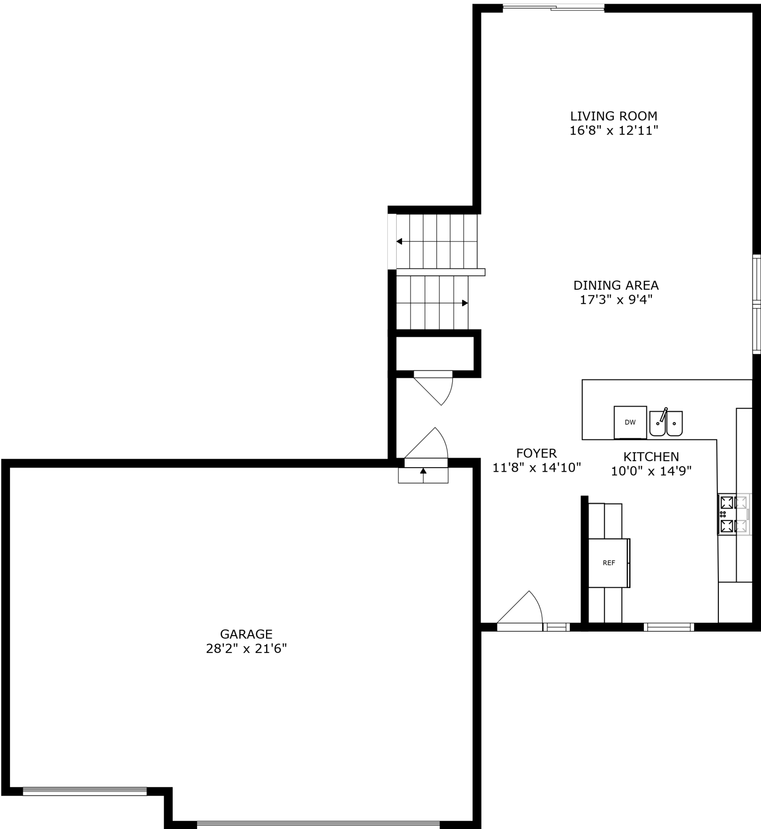
FLOOR 2
