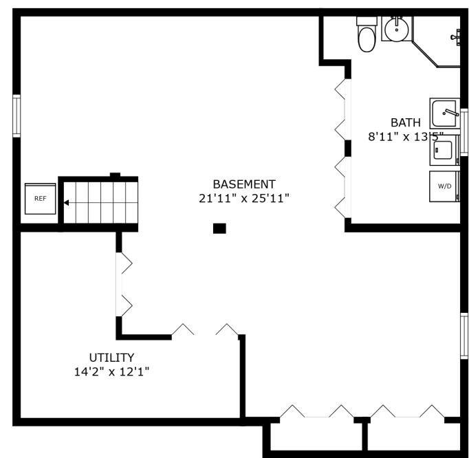
FLOOR 1
