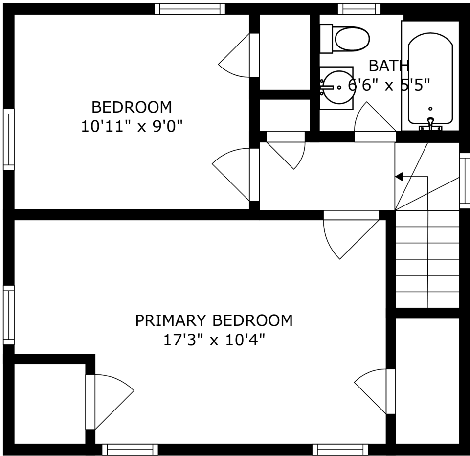
FLOOR 3
