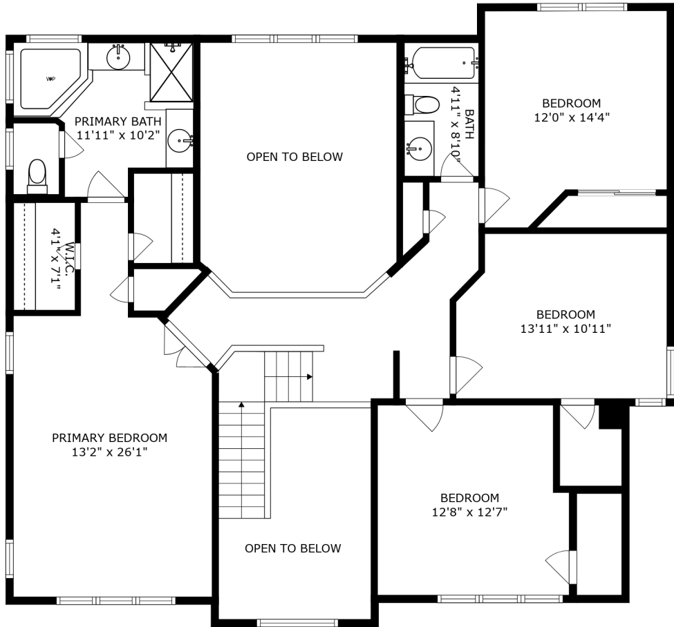
FLOOR 3
