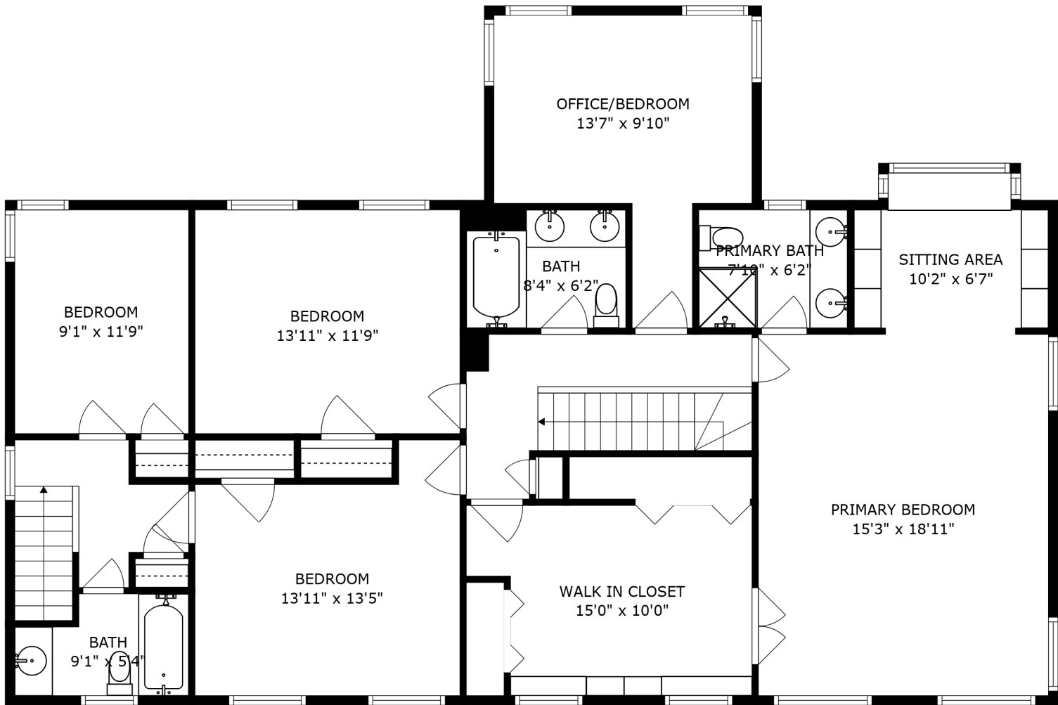
FLOOR 3
