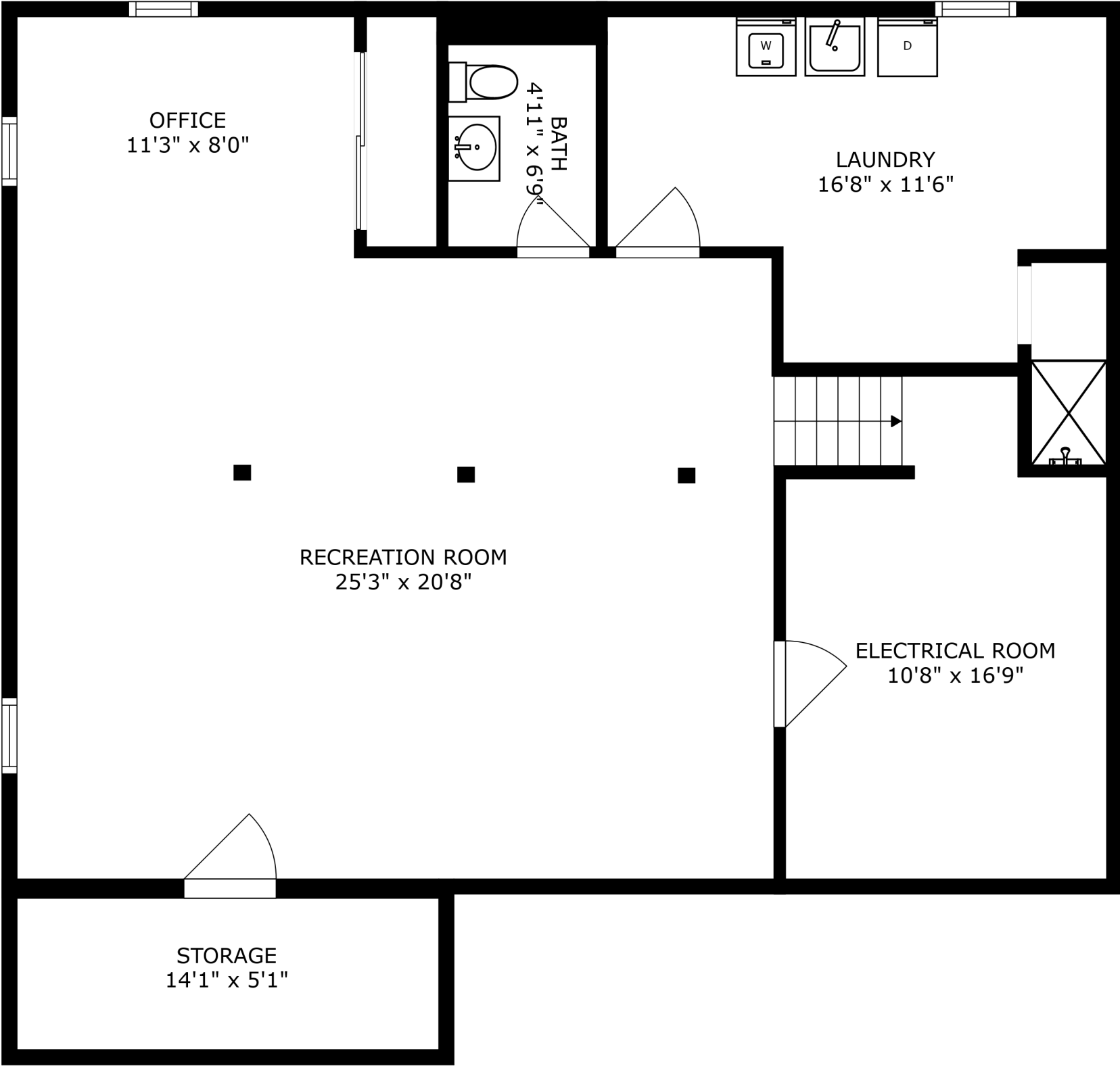
FLOOR 1
