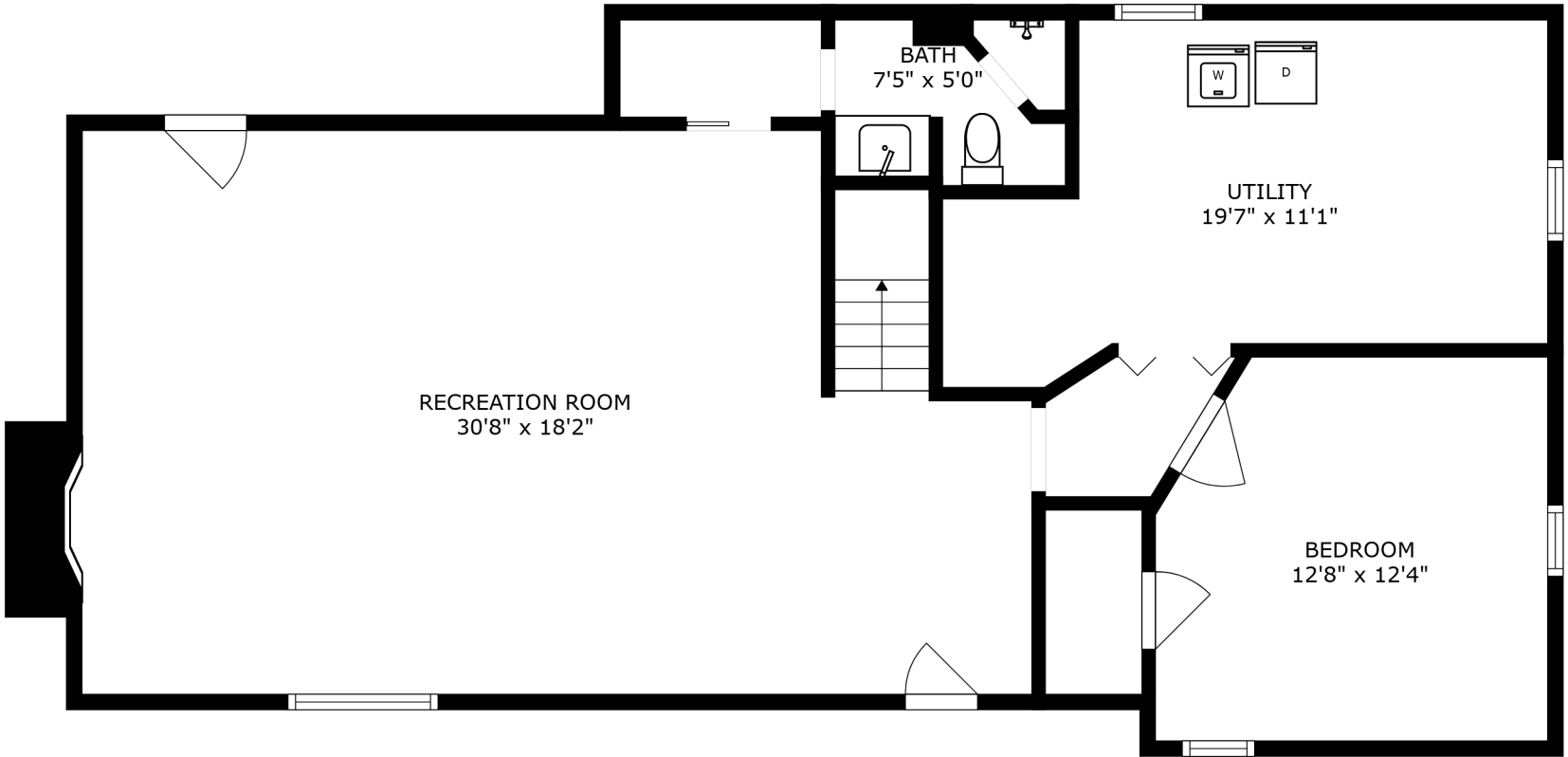
FLOOR 1
