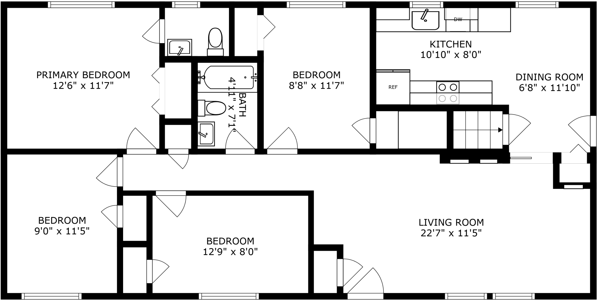
FLOOR 2
