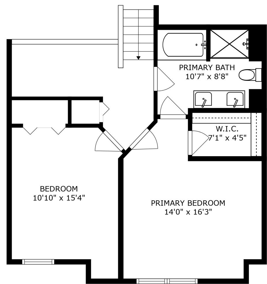
FLOOR 4
