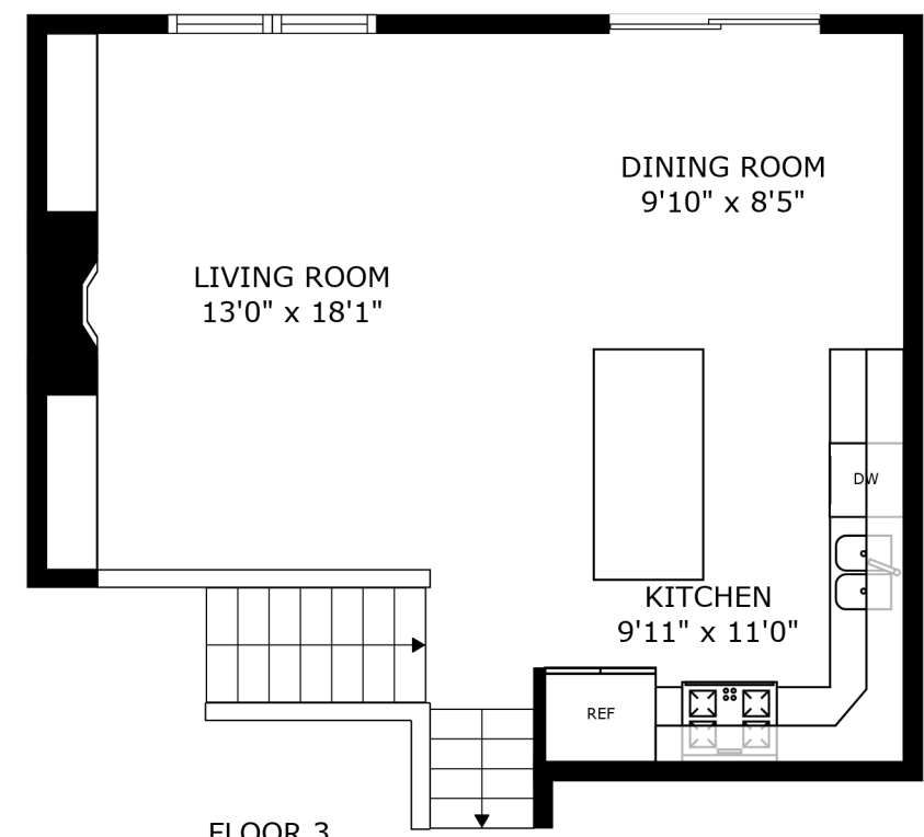
FLOOR 3
