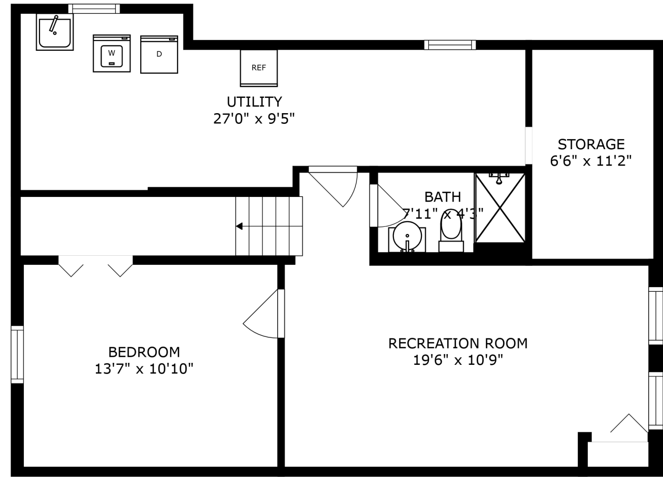
FLOOR 2
