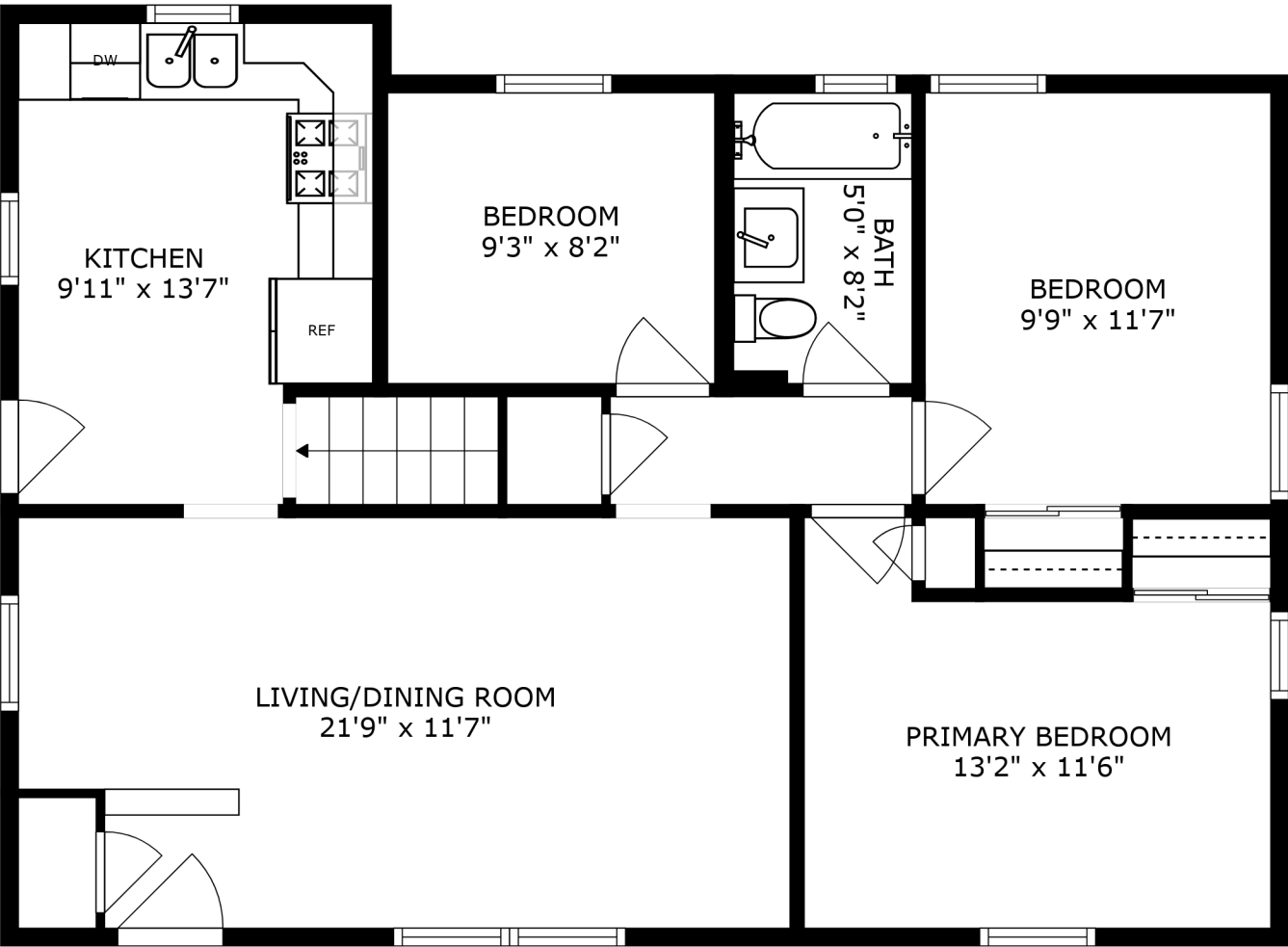
FLOOR 2
