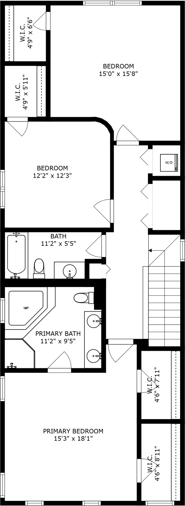
FLOOR 2
