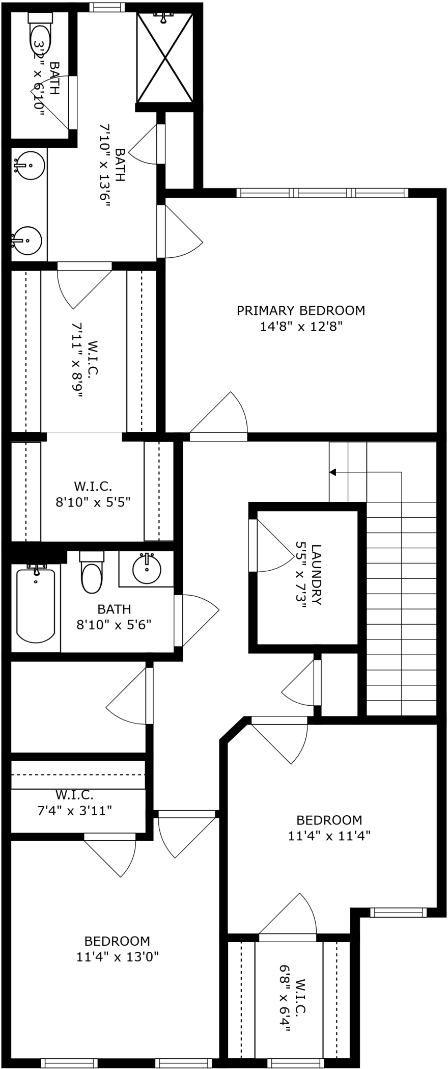
FLOOR 2
