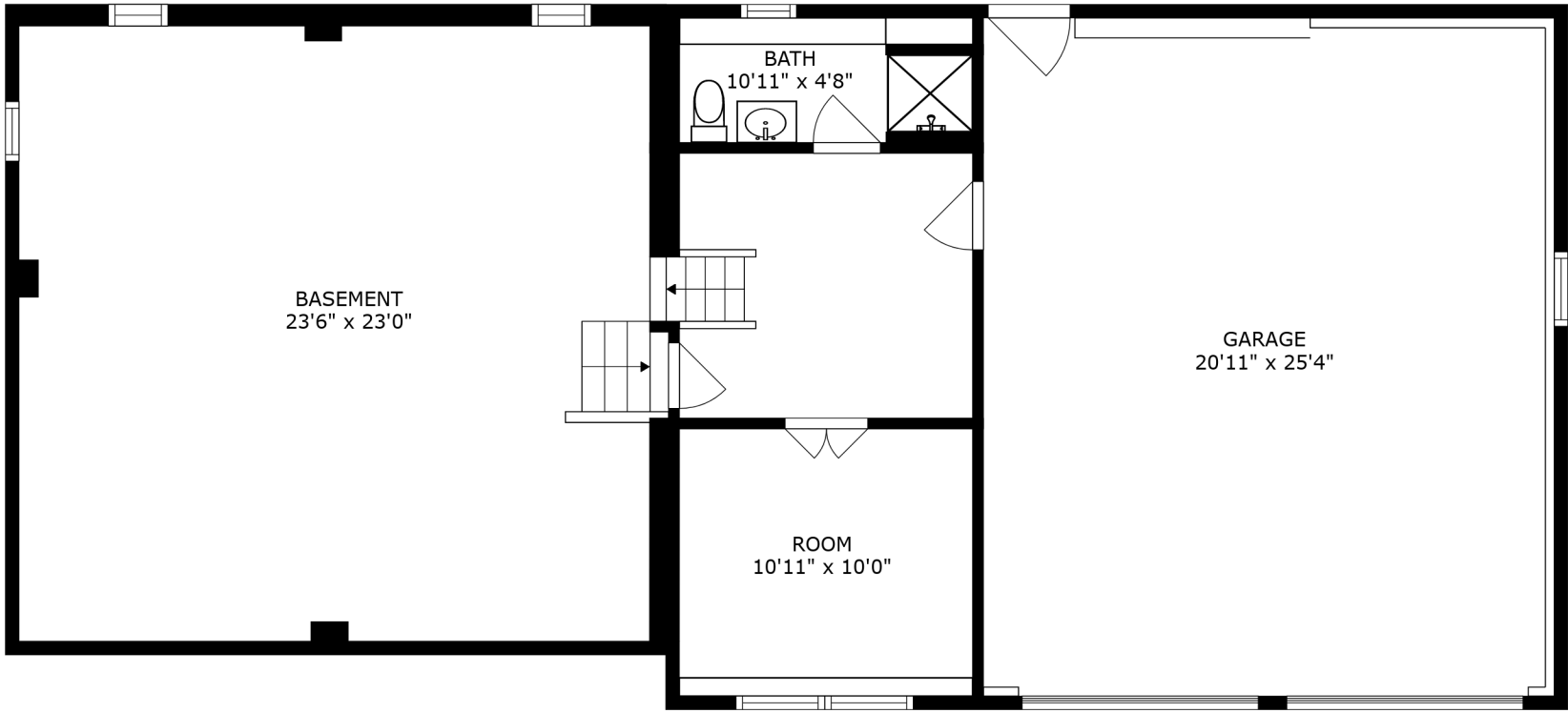
FLOOR 1
