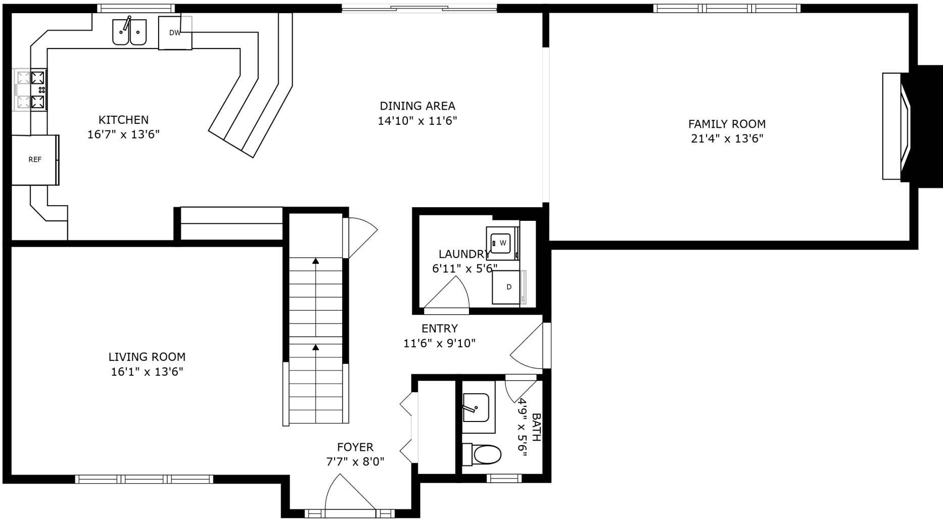
FLOOR 2
