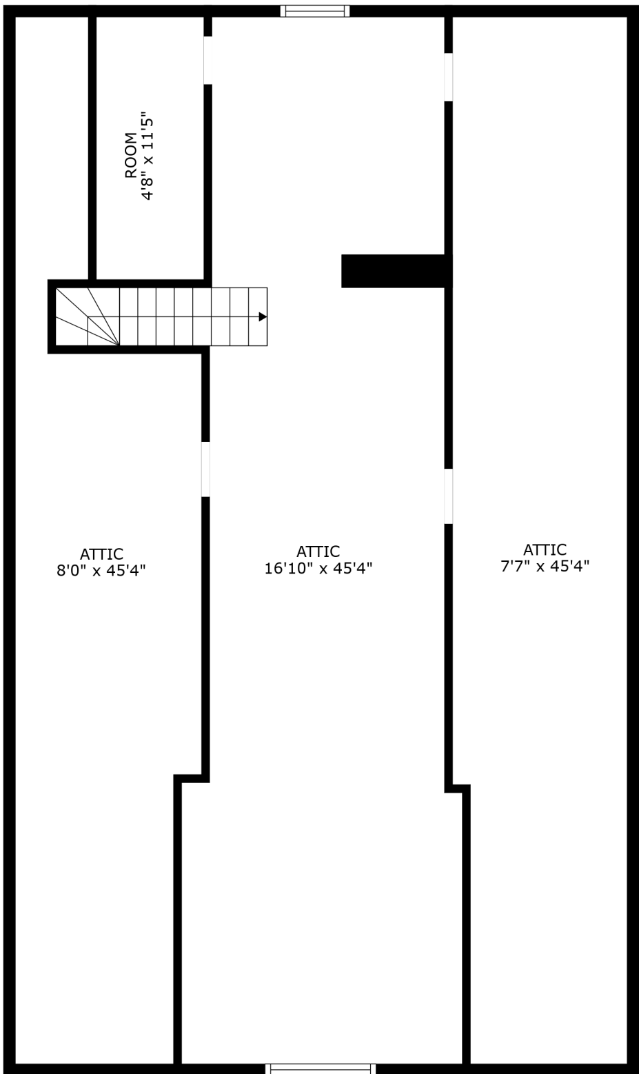
FLOOR 3
