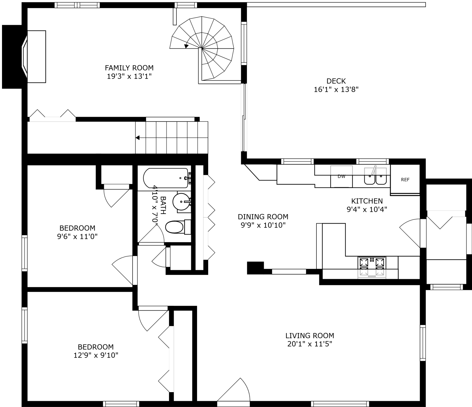
FLOOR 2
