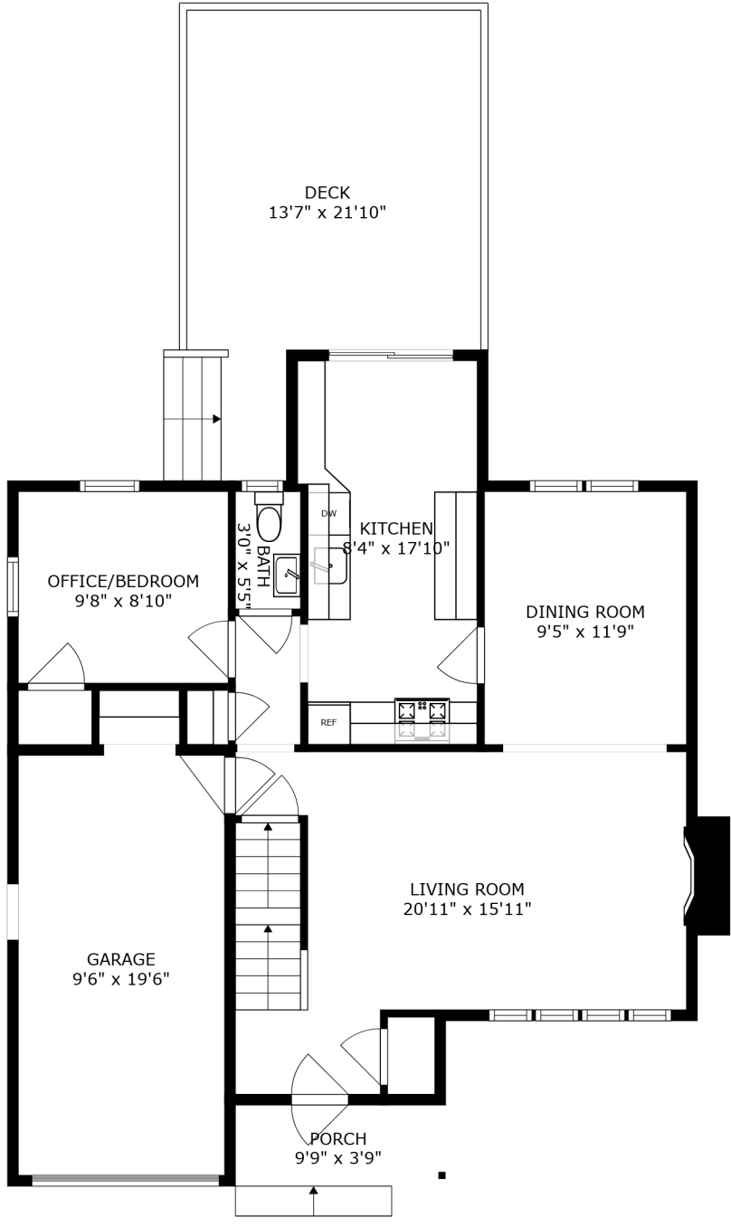
FLOOR 2
