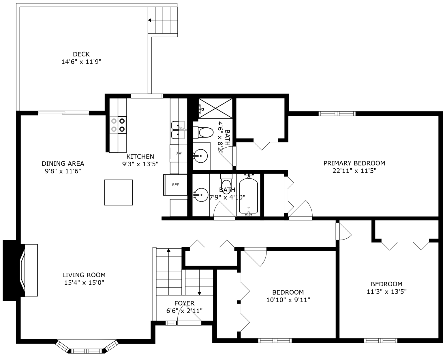
FLOOR 2
