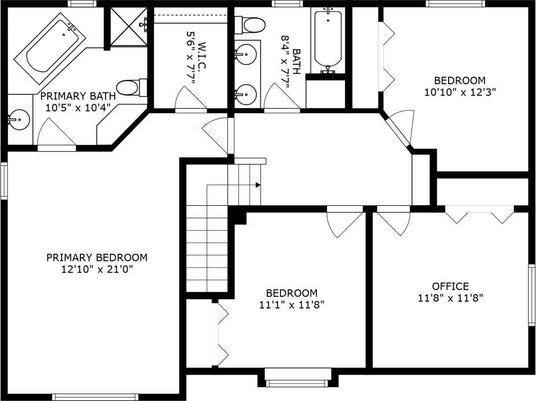
FLOOR 3
