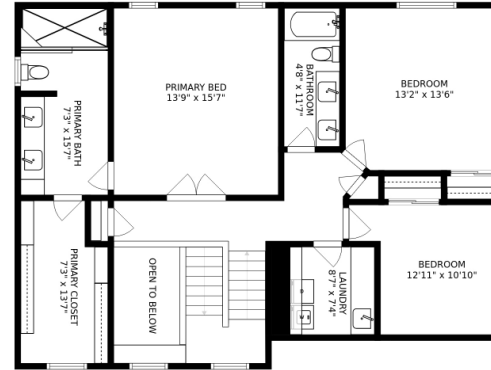
FLOOR 3
