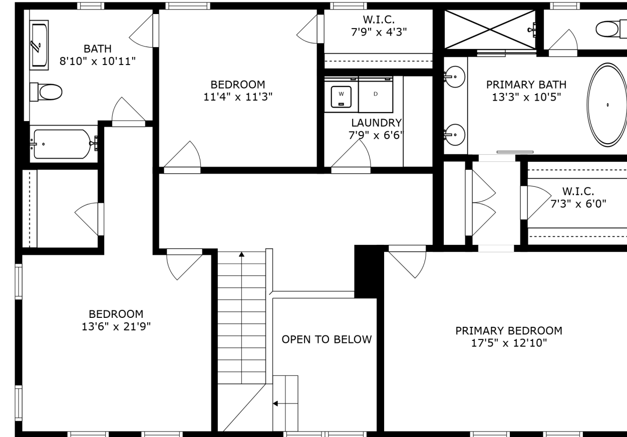
FLOOR 3
