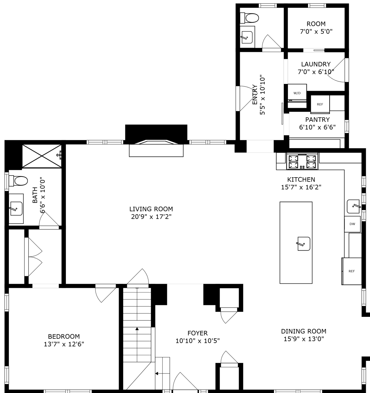
FLOOR 2
