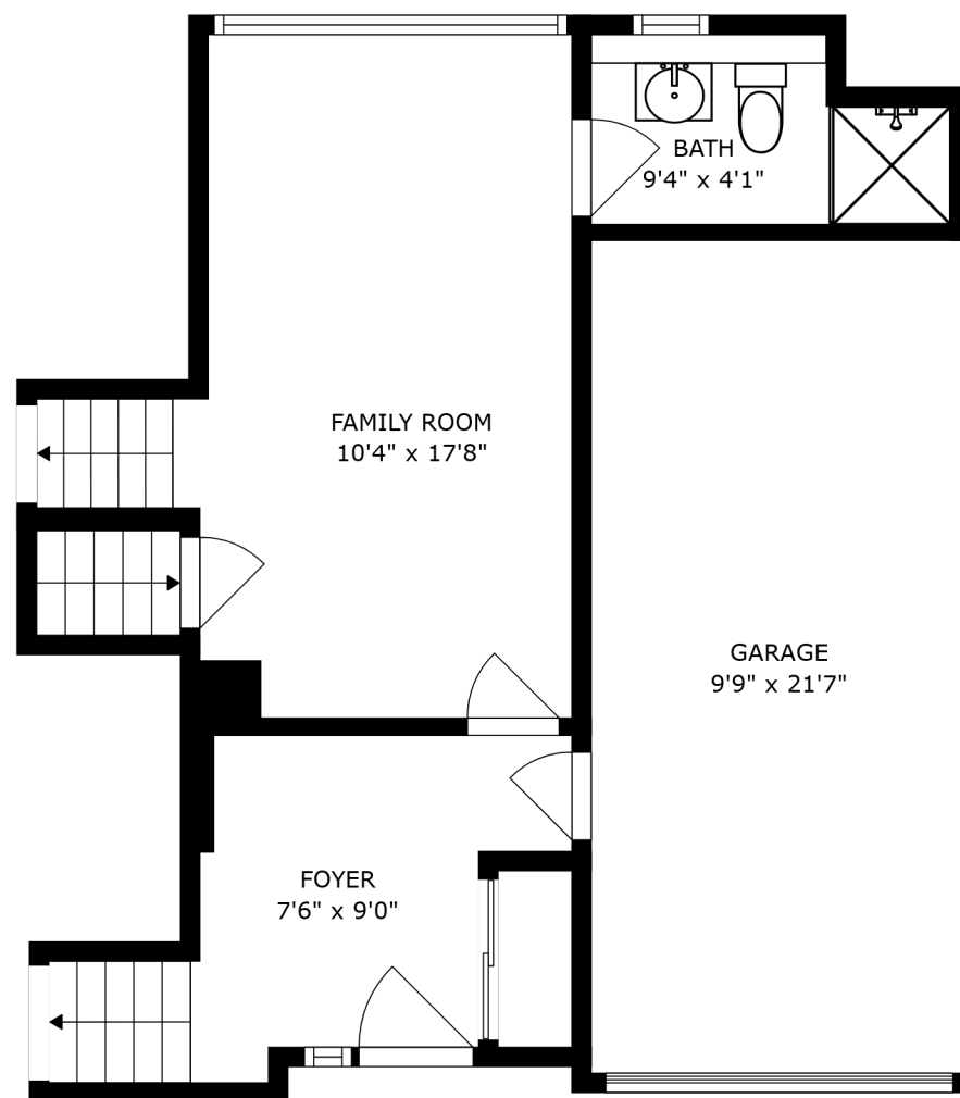
FLOOR 4
