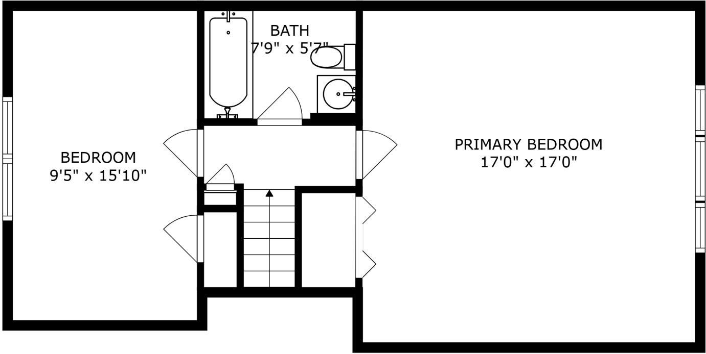
FLOOR 2
