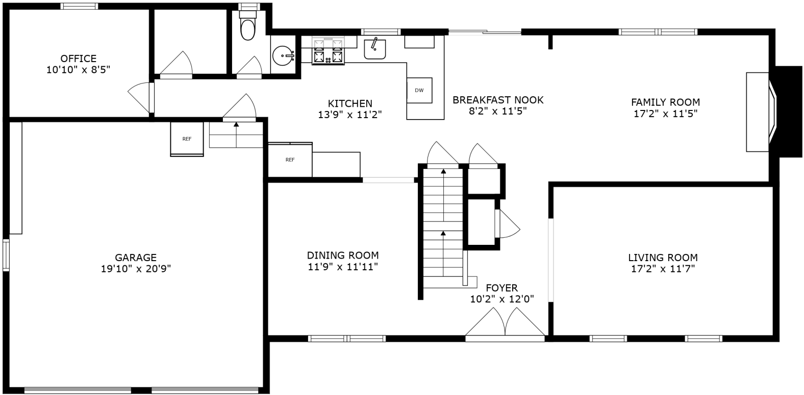
FLOOR 2
