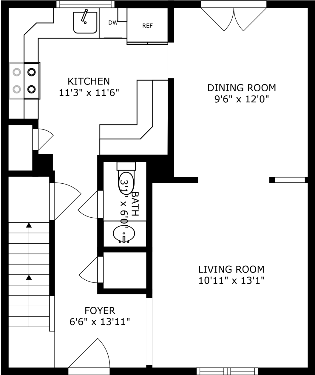
FLOOR 2
