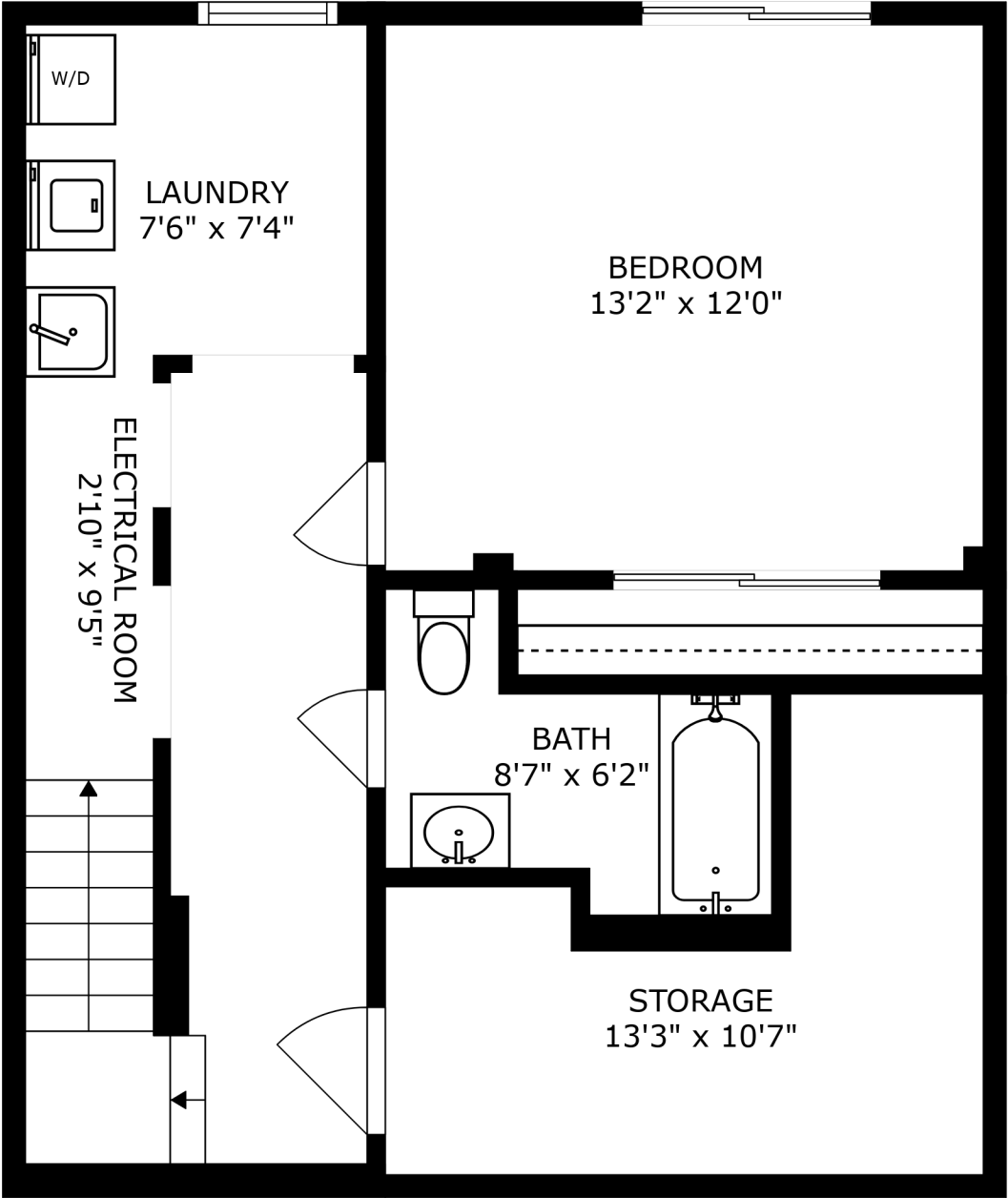
FLOOR 1
