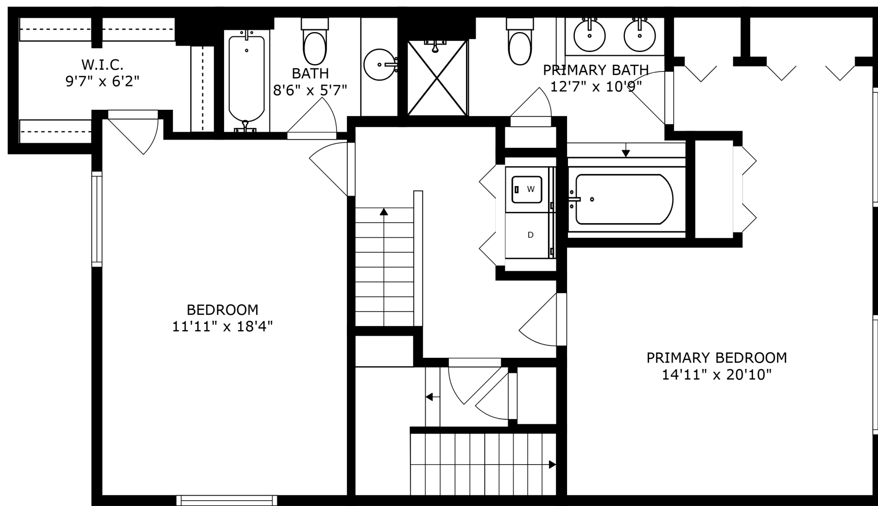
FLOOR 2
