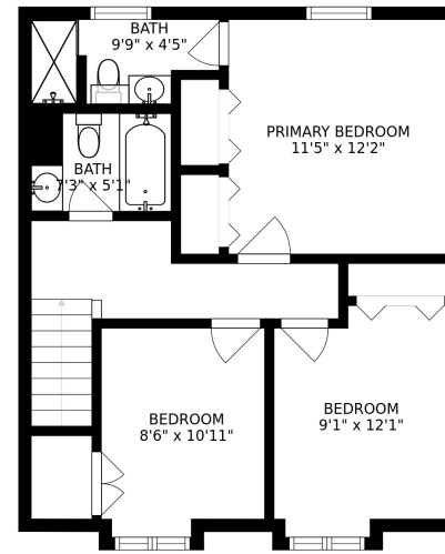
FLOOR 3
