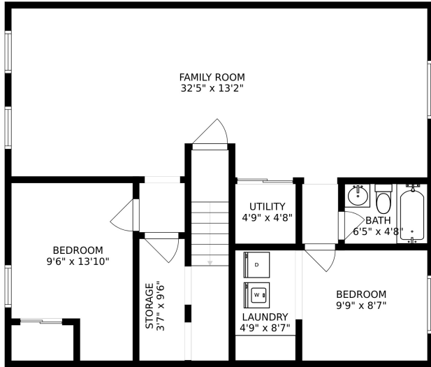
FLOOR 1
