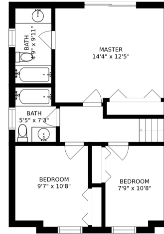
FLOOR 3
