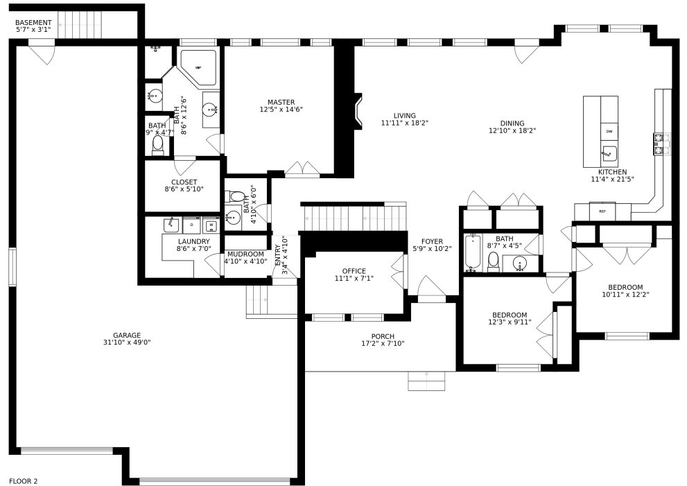
FLOOR 2
