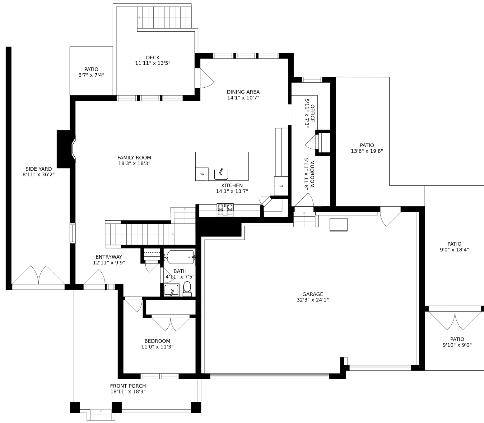
FLOOR 2
