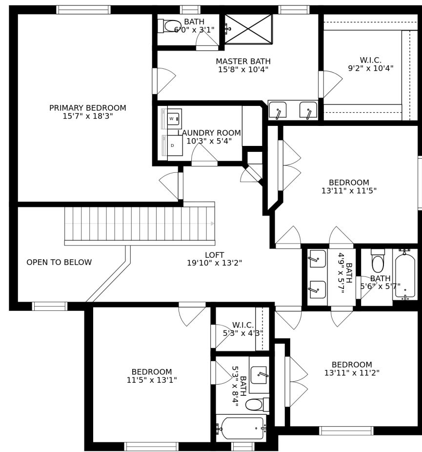
FLOOR 3
